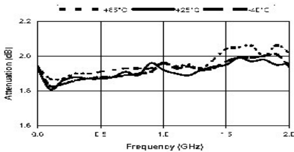
8 dB Bit vs. Temperature
