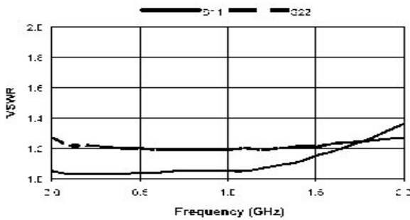
VSWR (S11, S22), 8 dB Bit
